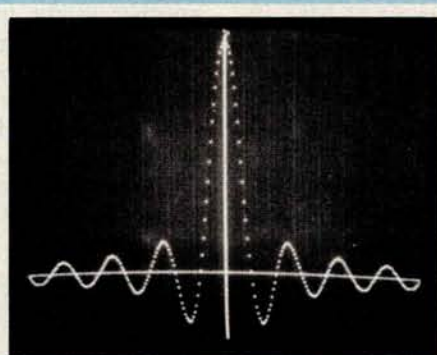
DAMPED FUNCTION; \sin(x)/x [-25, 25]
