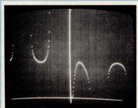
Y = (\sin(x))^{(1/x)} [-10, 10]
