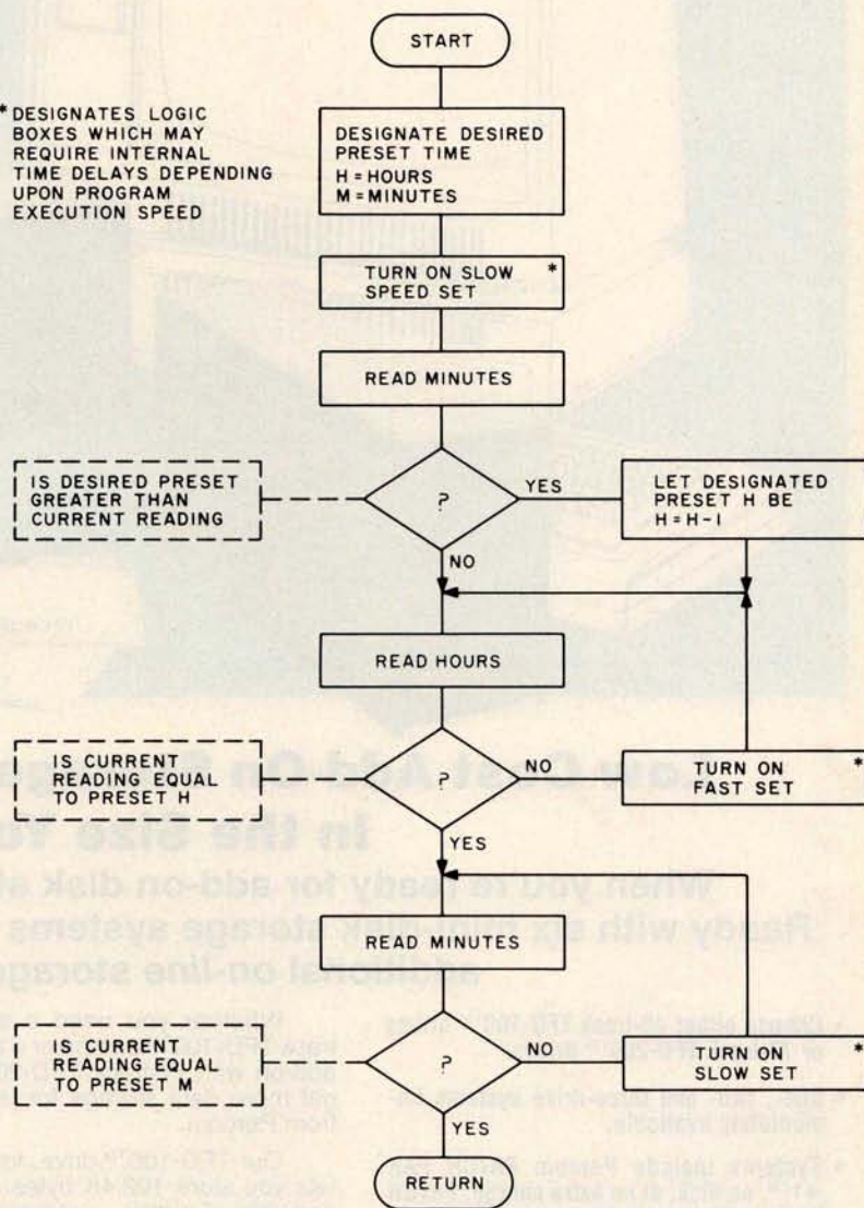
Figure 8: Flowchart for the automatic reset routine.
