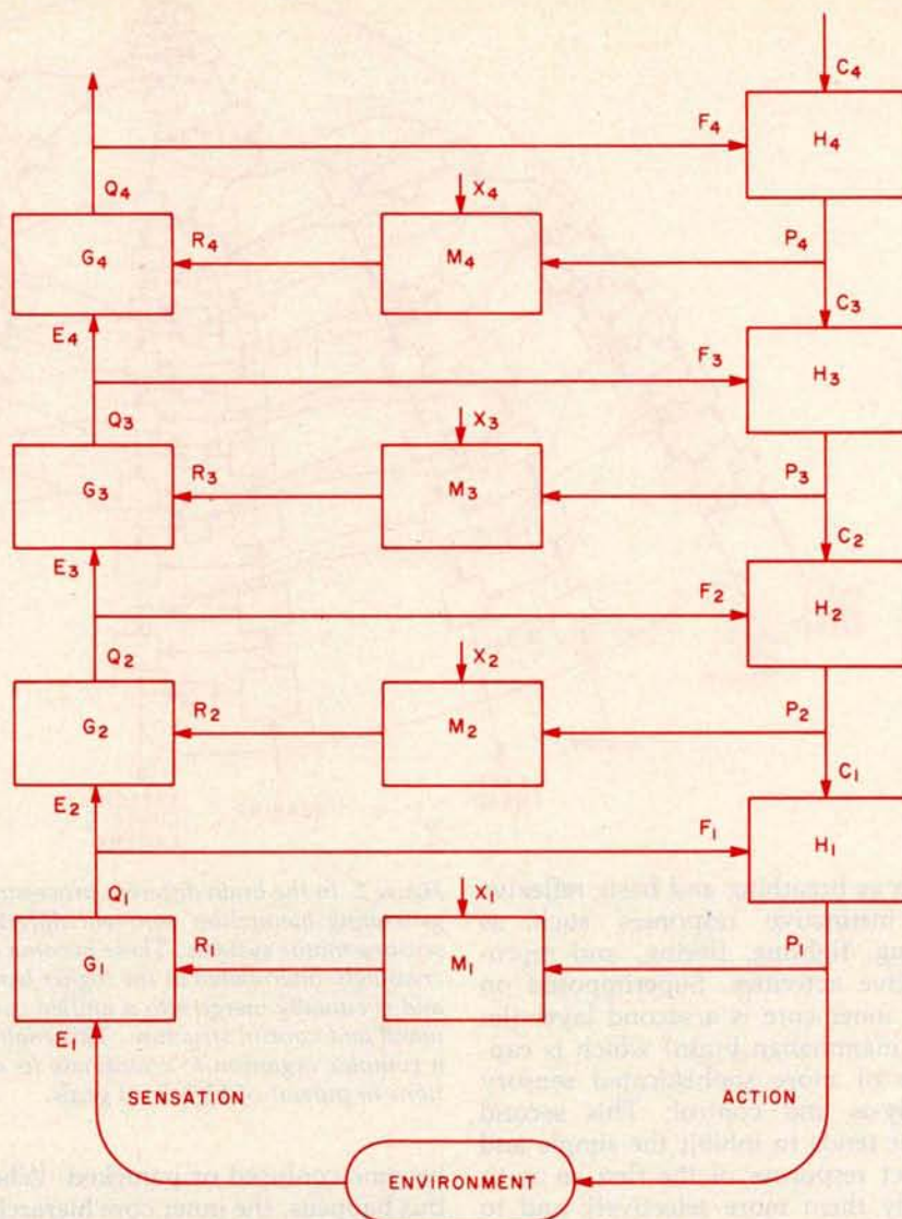
Figure 1: A crosscoupled, processing-generating hierarchy. The H modules decompose input goals C into output subgoals P using feedback F. The M modules recall expected sensory data R which is compared with observed sensory experiences E. The G modules recognize sensory patterns Q and compute feedback errors F.
