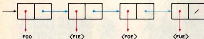
Figure 4: Storage representation of an object created by MK-FOO.
