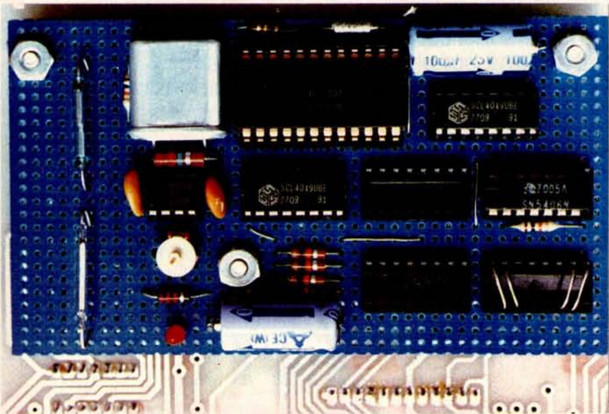
Photo 1: A prototype board of real-time clock mounted on the back of an existing parallel I/O (input/output) board. Two reed switches on the left side of the board are for manual setting of the clock. The empty sockets are used for the particular application for which this board was designed, a home security system.
