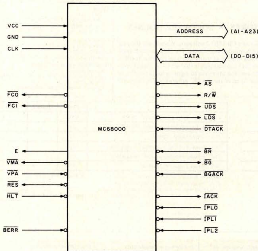
Figure 1: Pin assignments for the Motorola 68000 package. A description of the functions of the different pins is found in table 1. Figure reproduced courtesy of Motorola Semiconductor Products Inc.
