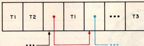
Figure 3: Paged partitions with tagged pointers: a pointer to an object of the type T2 and the representation of the integer 347.
