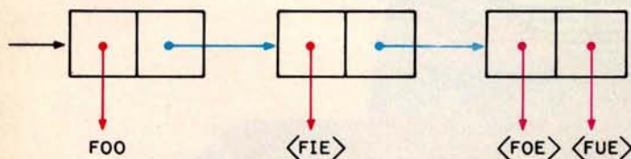
Figure 5: Storage representation of an object created by MK=FOO.
