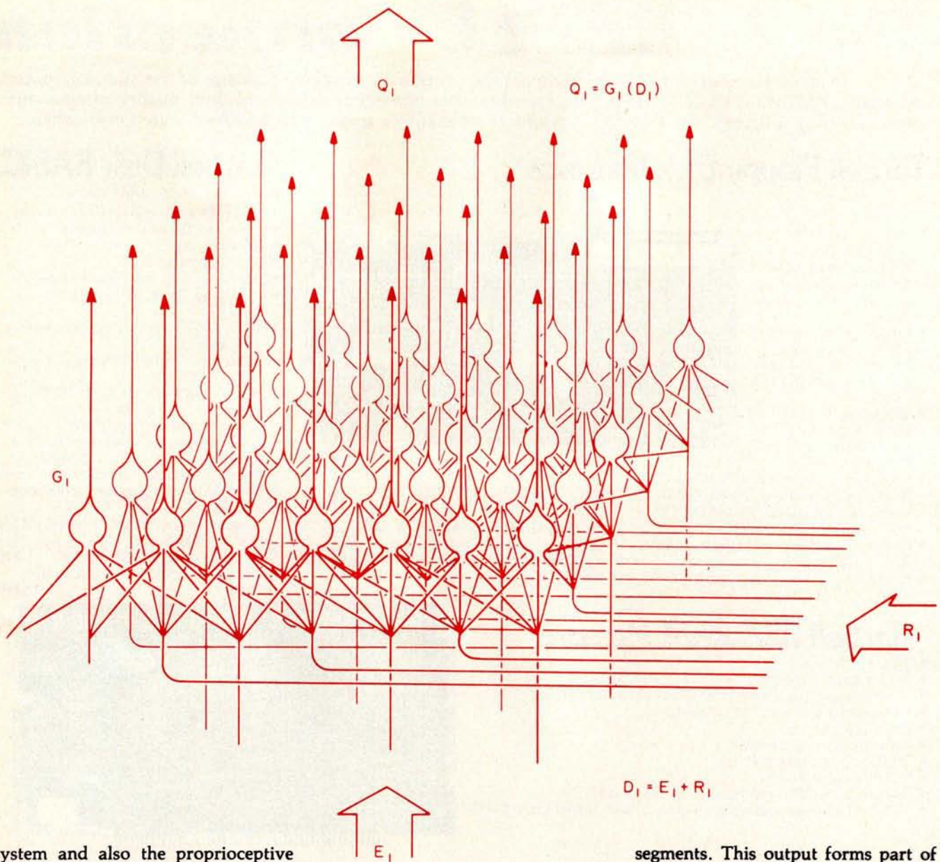
Figure 5: A two-dimensional array of sensory-processing Cerebellar Model Arithmetic Computers such as might exist in the visual system. The observed sensory image E_1 plus the prediction vector R_1 enters and is recognized by the operator G_1 as a pattern. The vector R_1 may select one of many filter functions or provide an expected image or map to be compared against the observed image.
